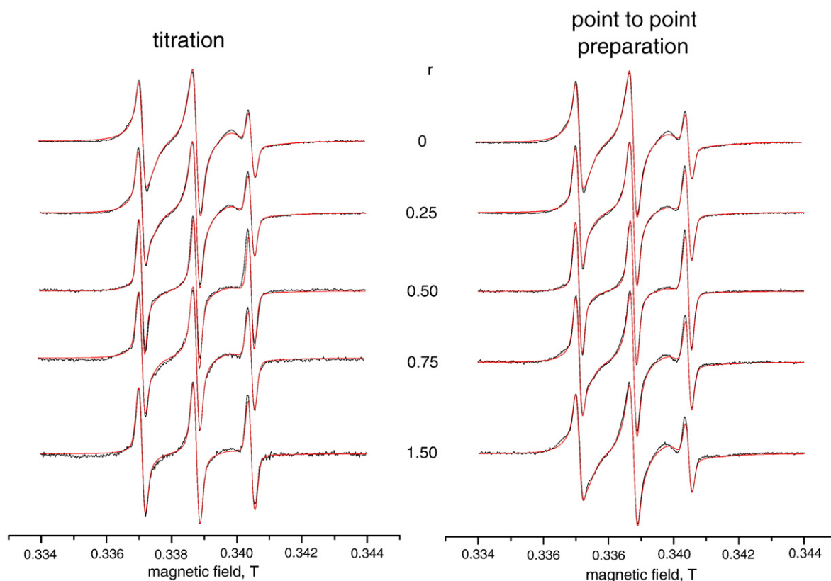
Fig. 2. Experimental (black line) and simulated (red line) ESR spectra at 298 K of CAT-12 inserted into dsAT/DOTAP/DOPE lipoplexes prepared by titration (left) and by point-to-point (right) at different r ratios. (For interpretation of the references to colour in this figure legend, the reader is referred to the web version of this article.)
