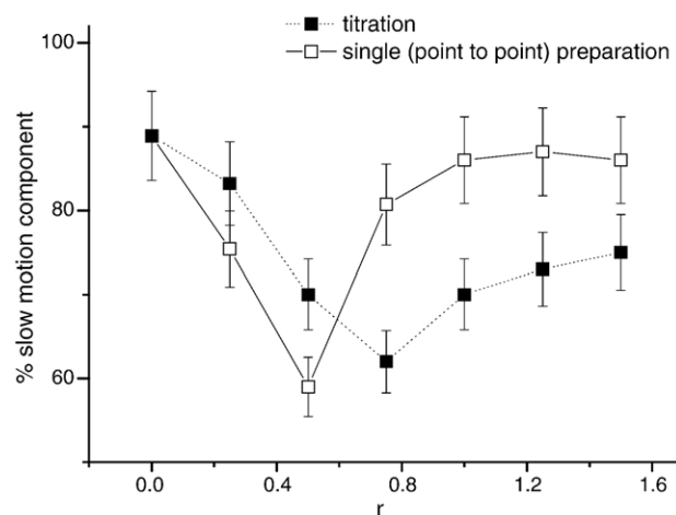
Fig. 3. Percentage of the slow moving species intensity used for the simulation of the ESR signals at different r for both preparation procedures described in the text. The error bars were determined by the fitting program.
