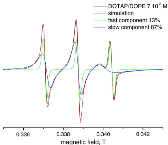
Fig. 1. Experimental (black line) and computed (red line) 298 K ESR spectra of CAT-12 nitroxide inserted into DOTAP/DOPE liposomes. The computed signal was the result of a sum of 13% fast moving species (green line) and 87% slow moving species (blue line). (For interpretation of the references to colour in this figure legend, the reader is referred to the web version of this article.)
